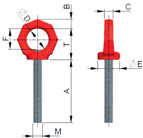
Pic. 5: Dimensioning
