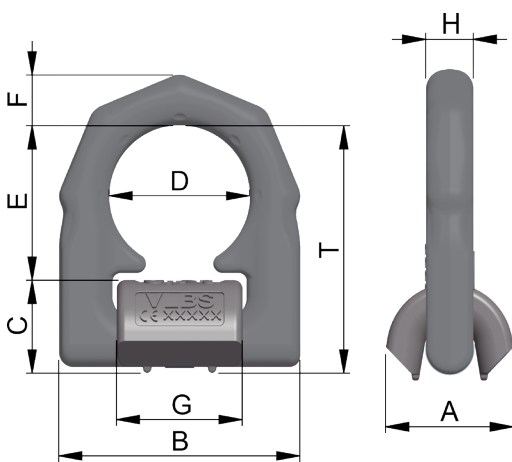
Pic. 4: Dimensioning
