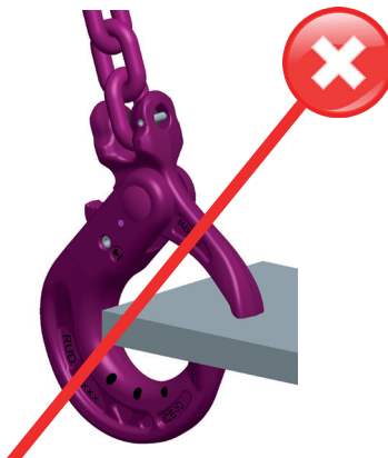
Pic. 15: No tip loading / not correctly locked
