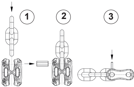
Pic. 3: Assembly of connecting pin
