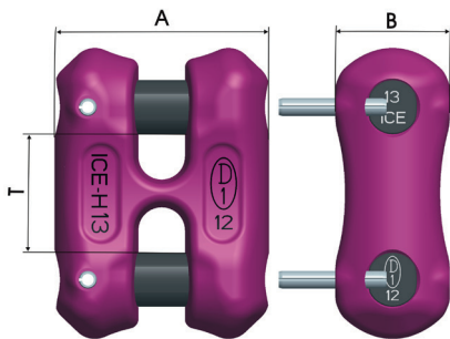
Pic. 5: Dimensioning
