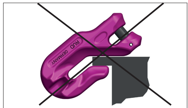
Pic.7: Forbidden attachment in components
