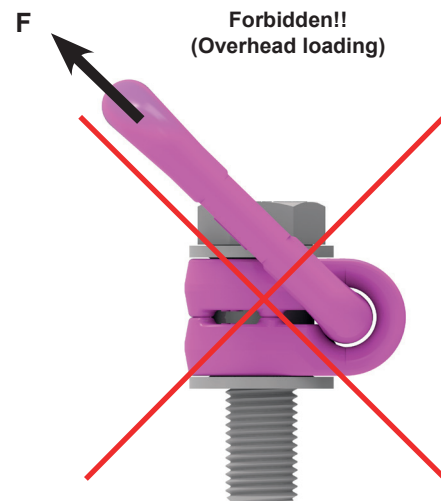
Pic. 8: Overhead loading
