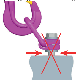
Pic. 4: The lashing point must be completely screwed in.
