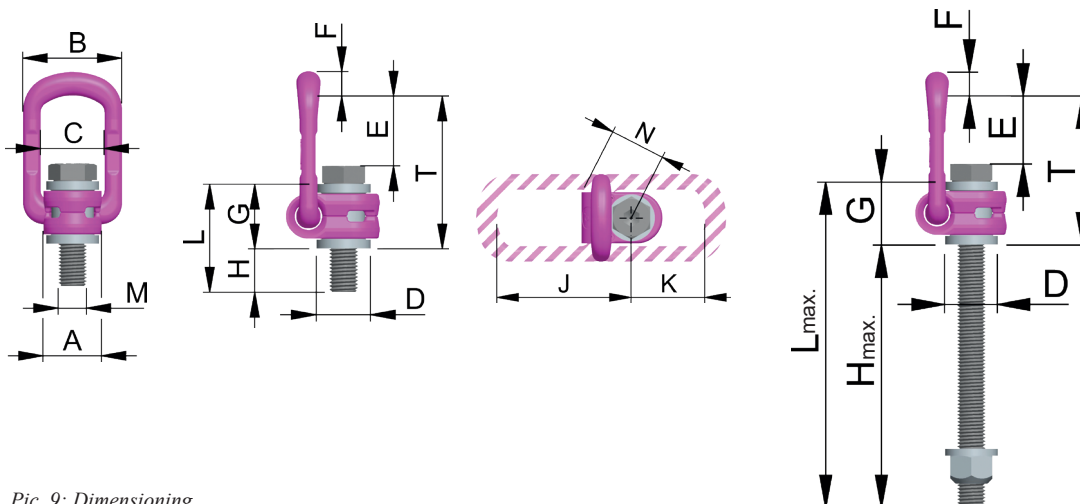
Pic. 9: Dimensioning
