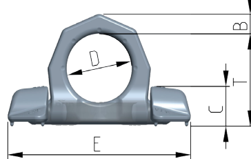
Pic. 10: Dimensioning LRBS (complete)
