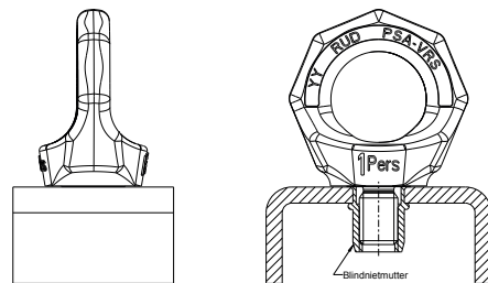
Pic. 1: Blind-rivet nut
