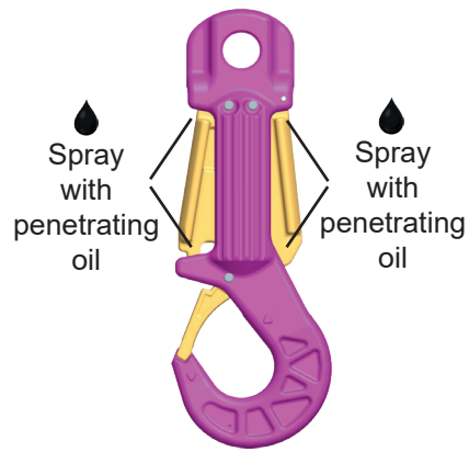
Pic. 10: Spray components with penetrating oil
