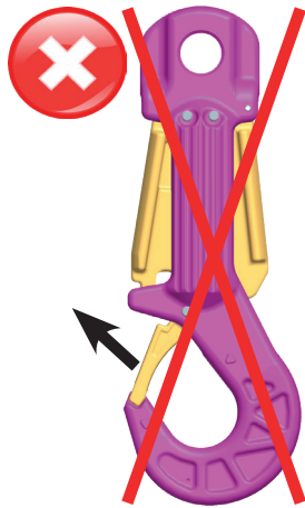
Pic. 9: Safety latch must not open manually.
