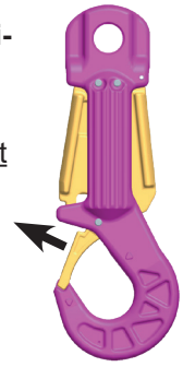
Pic. 7: Checking of safety latch
