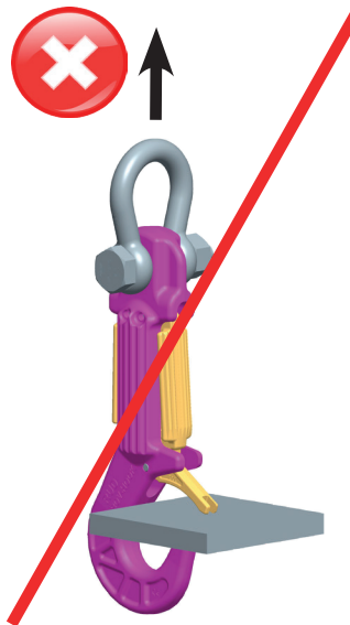
Pic. 14: ROV-HOOK loaded at the tip
