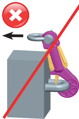
Pic. 12: ROV-HOOK loaded in the direction of the hook tip
