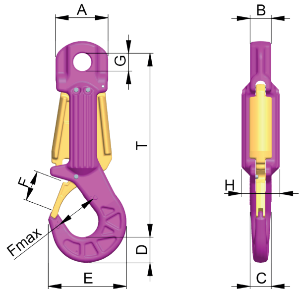
Pic. 15: Dimensions
