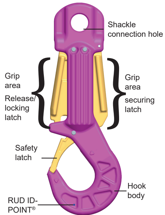
Pic. 8: Detailed illustration of the ROV-HOOK
