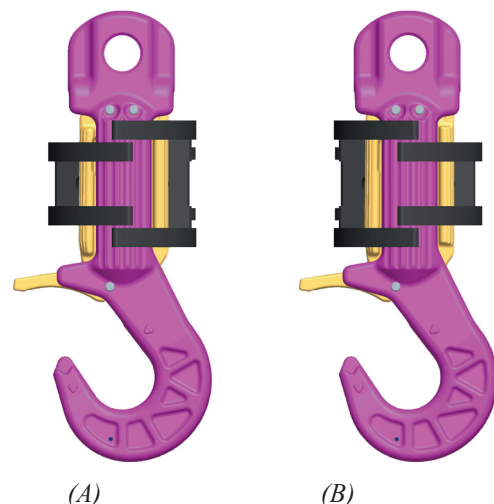
Pic. 4: Using the grippers
