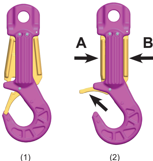
Pic. 6: The ROV-HOOK opening mechanism
