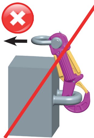
Pic. 13: Fig. ROV-HOOK loaded in the direction of the back of the hook
