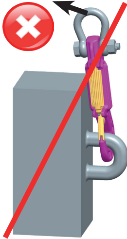
Pic. 11: ROV-HOOK with load at the side
