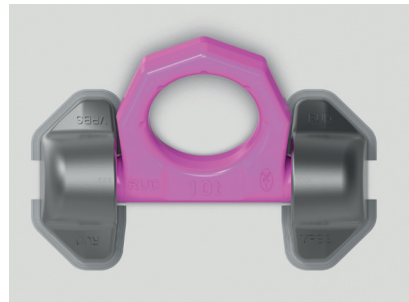
Pic. 4: Weld on welding block 2
