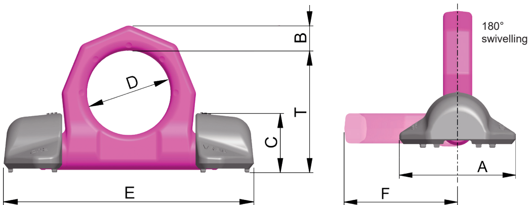
Pic. 10: Dimensioning
