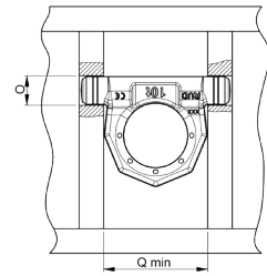
Pic. 8: Ring integrated in the construction:
