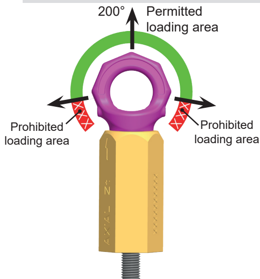
Pic. 4: Permissible loading area in the plain of the ring (green = permitted loading area)
