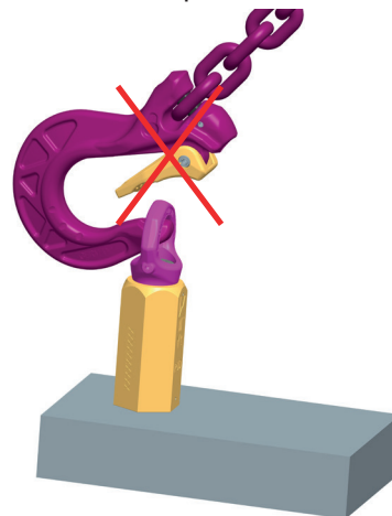
Pic. 2: Only use suitable lifting means for the hinging at the VRS with extension adaptors.
