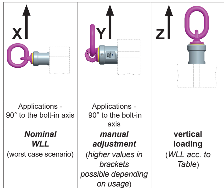
Pic. 9: Loading directions
