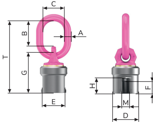
Pic. 8: Dimensioning
